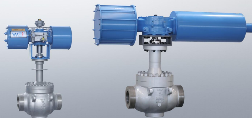
超低温上装式球阀 Cryogenic Top Mounted Ball Valve 超低温高压上装式球阀 Cryogenic and High Pressure Top Mounted Ball Valve
