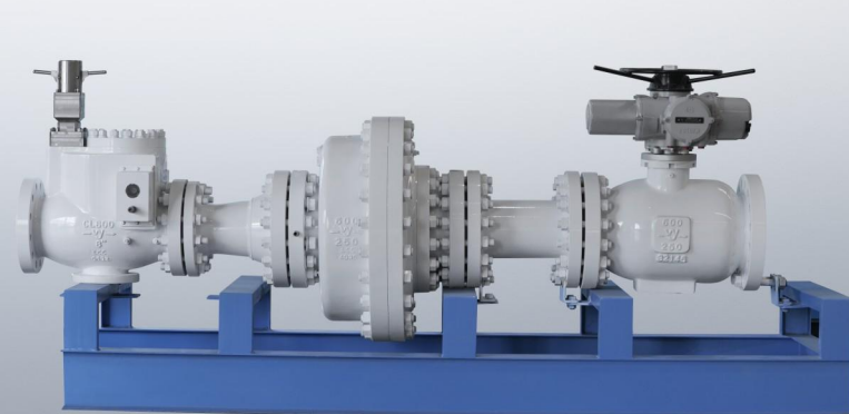
天然气调压撬 Natural Gas Regulator Skid
