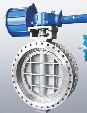
气动三偏心蝶阀 Pneumatic triple eccentric Butterfly Valve
