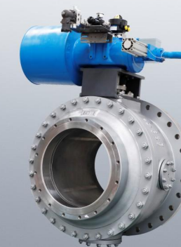
锅盖球阀 Digester feed ball valve
