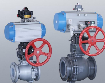
衬塑球阀 Anti Corrosion Lined Plastic Ball Valve
