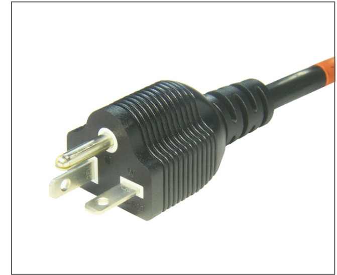
• NEMA 6-20P Plug
