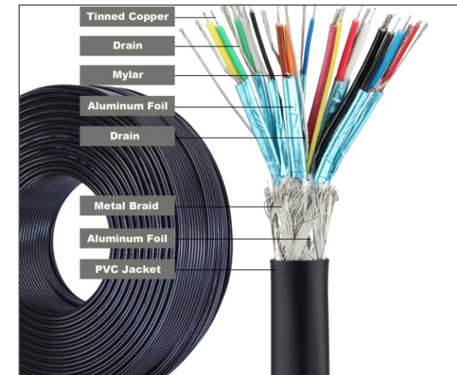
• USB High-frequency Data Cable (UL 2725, UI20276)
