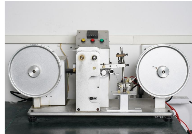
纸带耐磨测试仪 Paper tape abrasion resistance tester
