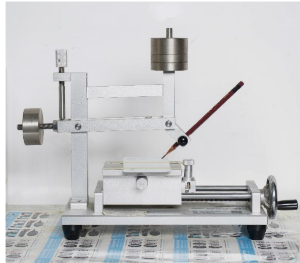
铅笔硬度测试仪 Pencil hardness tester
