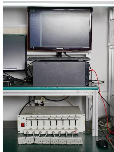
电池分容仪 Battery Capacity Analyzer
