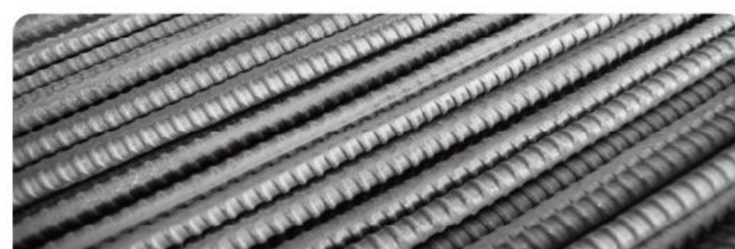
RFH-FW009F 热轧夹器螺杆 Hot Rolled Tie Rod 17mm Φ 17/Φ 22 1000, 1500, 2000, 2500, 3000, 4000, 6000mm ≥ 180KN
