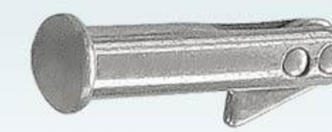
RFH-E004E 销子 Lock Pin 0.05kg Dia12.7X55mm
