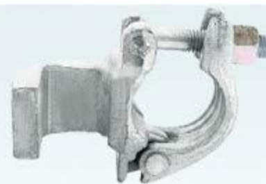
RFH-A076 防滑杠焊接L板扣件 Coupler With Welded L-Plank 48.3mm 1.15kg
