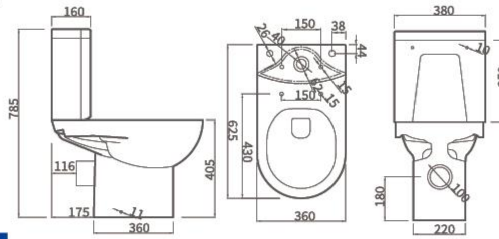
FTZ-6612 Washdown Two-piece toilet Rimless flush Size: 625x380x785mm P-trap: 180mm Roughing-in
