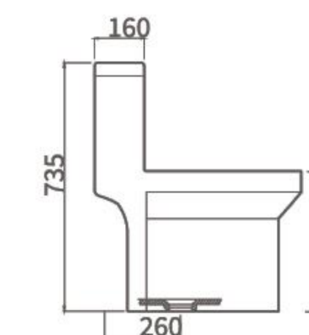
FTO-2401 Siphonic One-piece toilet Size: 620×335×735mm S-trap, 260mm Roughing-in
