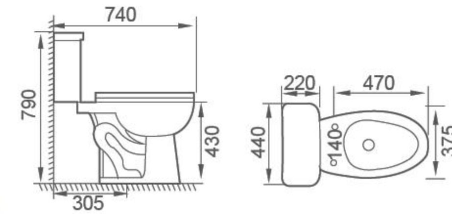
FTZ-1903 Siphonic Two-piece Toilet Size: 740×440×790mm S-trap, 305mm Roughing-in
