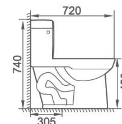
FTO-8848 Siphonic One-piece toilet Size: 720×367×740mm S-trap, 305mm Roughing-in
