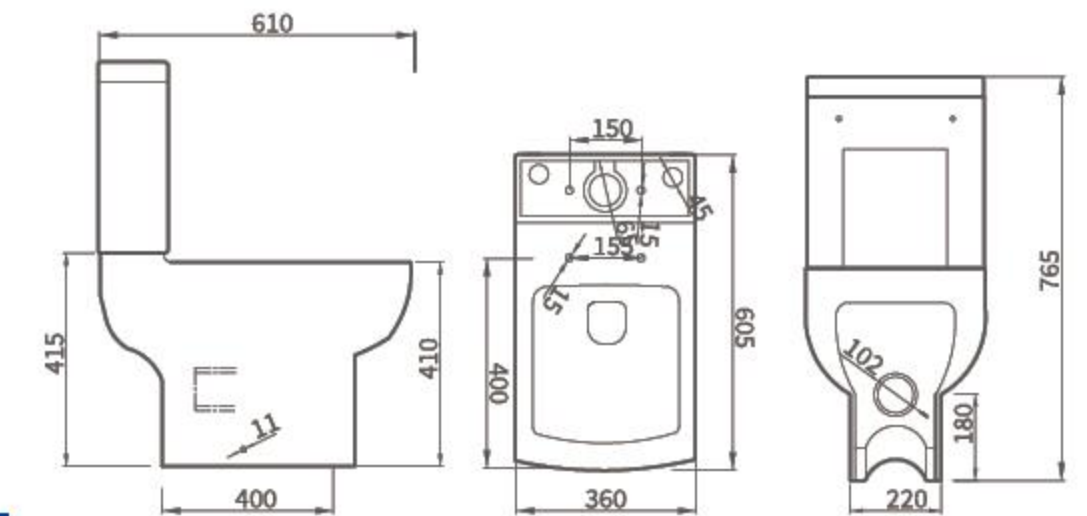
FTZ-6606 Washdown Two-piece toilet Size:610x360x765mm P-trap:180mm Roughing-in
