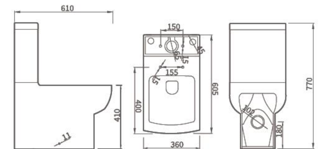
FTZ-6606D Washdown Two-piece toilet Size:610x360x770mm P-trap:180mm Roughing-in
