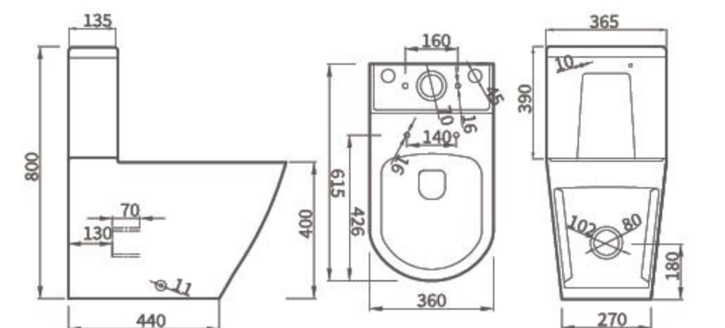
FTZ-2403 Washdown Two-piece toilet Tornado Flush Size: 615×365×800mm P-trap, 180mm Roughing-in
