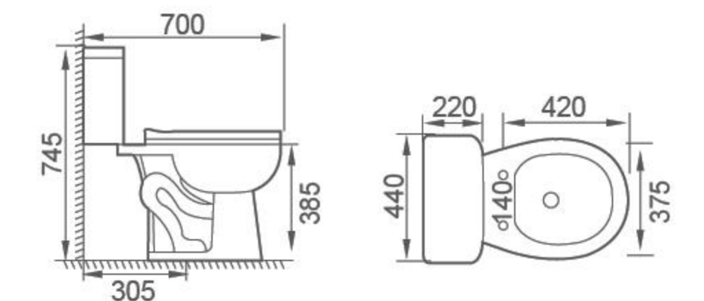
FTZ-1901 Siphonic Two-piece Toilet Size: 700×440×745mm S-trap, 305mm Roughing-in
