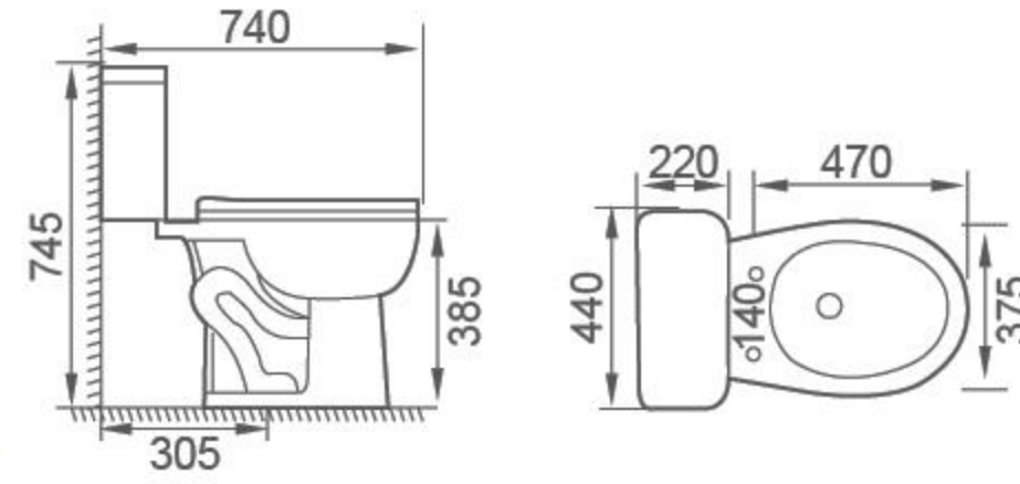
FTZ-1902 Siphonic Two-piece Toilet Size: 740×440×745mm S-trap, 305mm Roughing-in
