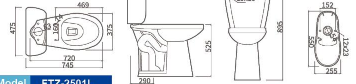
FTZ-2501L Siphonic Two-piece toilet Size: 745×475×895mm S-trap, 290mm Roughing-in
