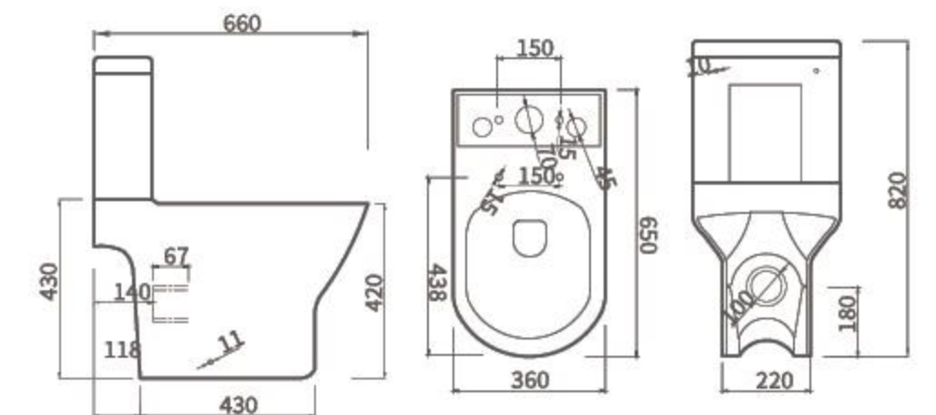
FTZ-2402 Washdown Two-piece toilet Tornado Flush Size: 660×360×820mm P-trap, 180mm Roughing-in
