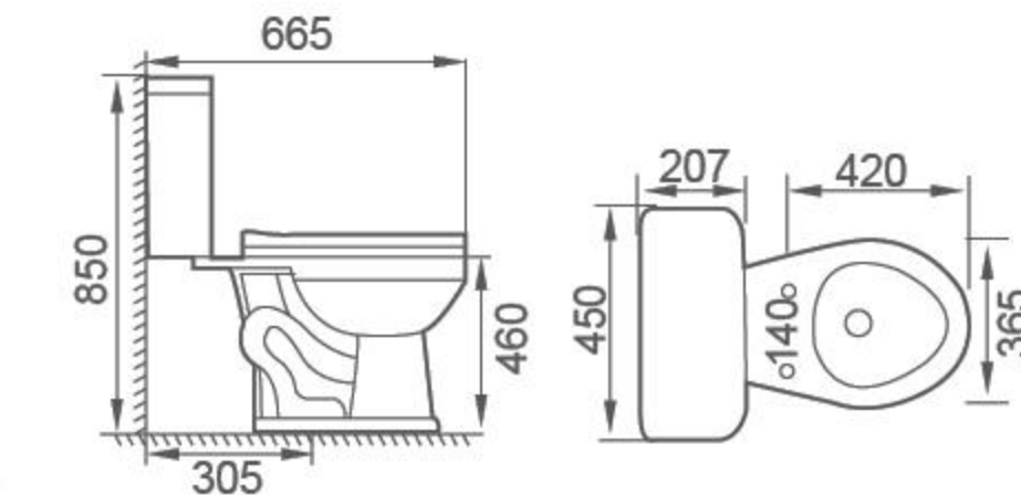
FTZ-3430R Siphonic Two-piece toilet Comfort Height Size: 665×450×850mm S-trap, 305mm Roughing-in
