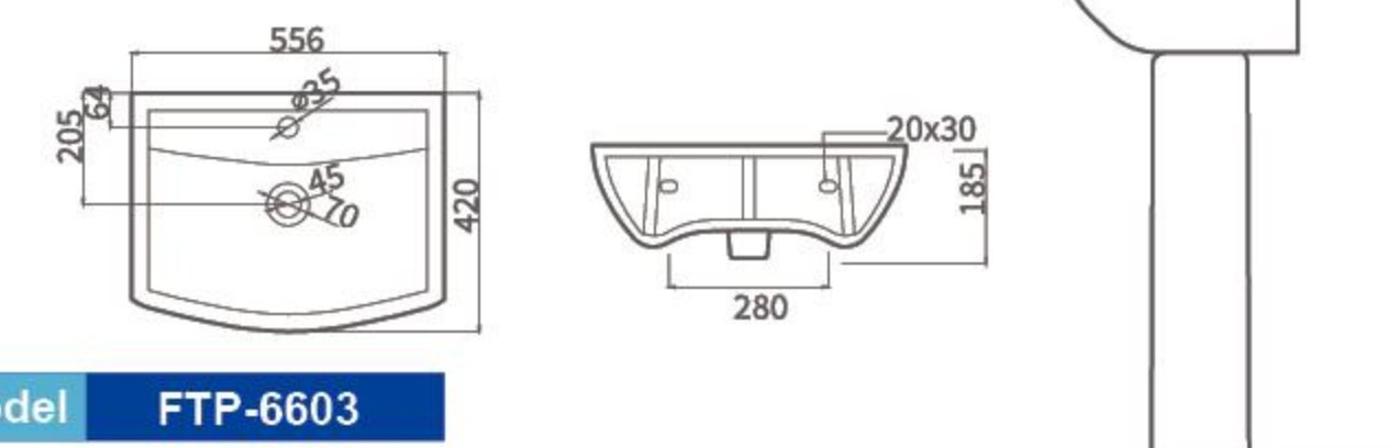
FTP-6603 Basin with full pedestal Size: 556×420×868mm
