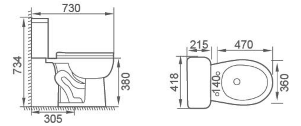
FTZ-0425D Siphonic Two-piece Toilet Size: 730×418×734mm S-trap, 305mm Roughing-in
