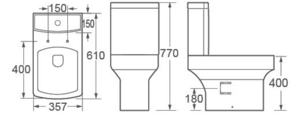
FTZ-6602 Washdown Two-piece toilet Rimless flush Size: 610×357×770mm
