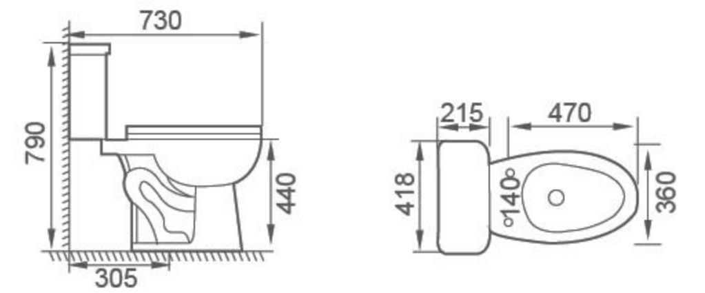
FTZ-0425HS Siphonic Two-piece Toilet Size: 730×418×790mm S-trap, 305mm Roughing-in
