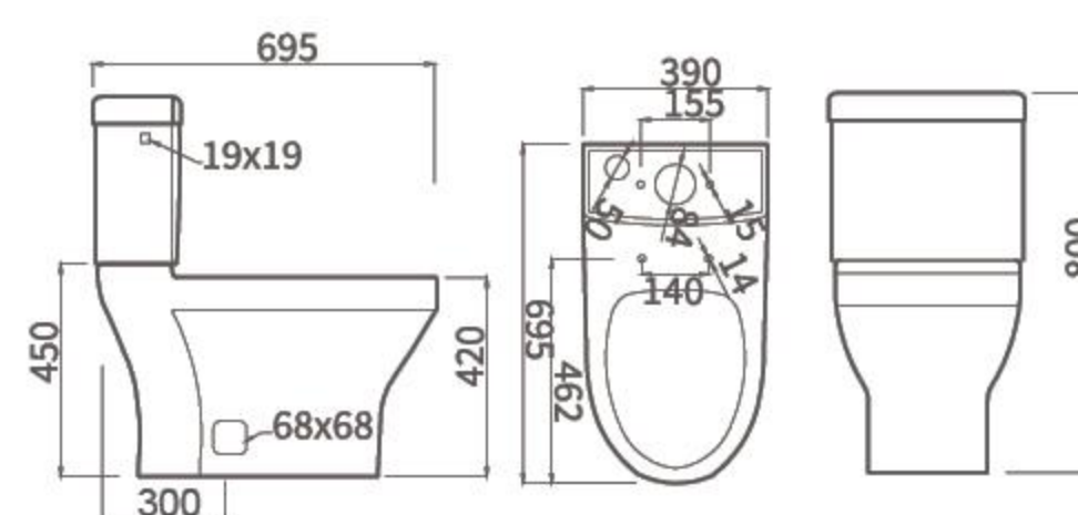
FTZ-2405 Siphonic Two-piece toilet Tornado Flush Size: 695×390×800 S-trap, 300mm Roughing-in
