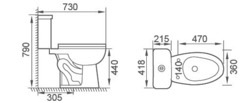
FTZ-0425HD Siphonic Two-piece Toilet Size: 730×418×790mm S-trap, 305mm Roughing-in
