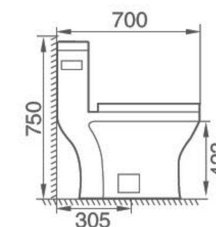
FTO-8004 Siphonic One-piece toilet Size: 700×364×750mm S-trap, 305mm Roughing-in
