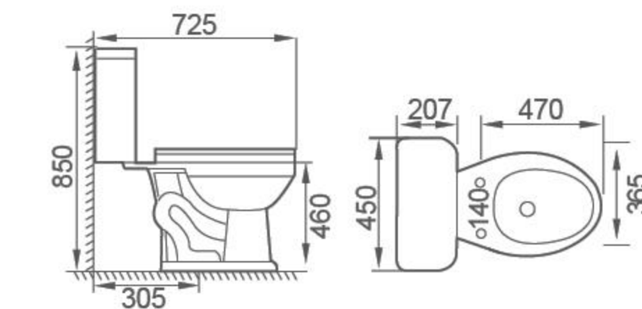
FTZ-3430 Siphonic Two-piece toilet Comfort Height Size: 725×450×850mm S-trap, 305mm Roughing-in
