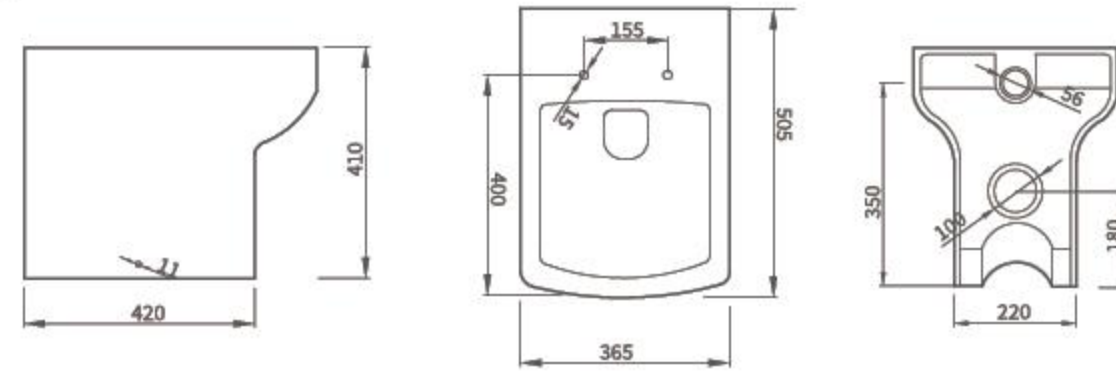
FTZ-6606X Washdown Floor standing BTW toilet Size:505x365x410mm P-trap:180mm Roughing-in
