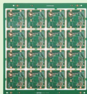
投影仪小家电产品 Projector Small Appliances,0.4mm finished thickness
