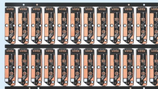
单面铝基绝缘孔工艺，主要用于安防产品 Single-sided MPCB insulation hole process, Mainly used for security products
