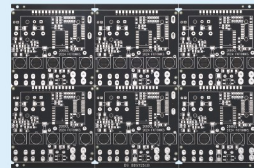
双面碳油板，主要用于按键类主板 Double-sided carbon oil plate, Mainly used for keypad motherboards.
