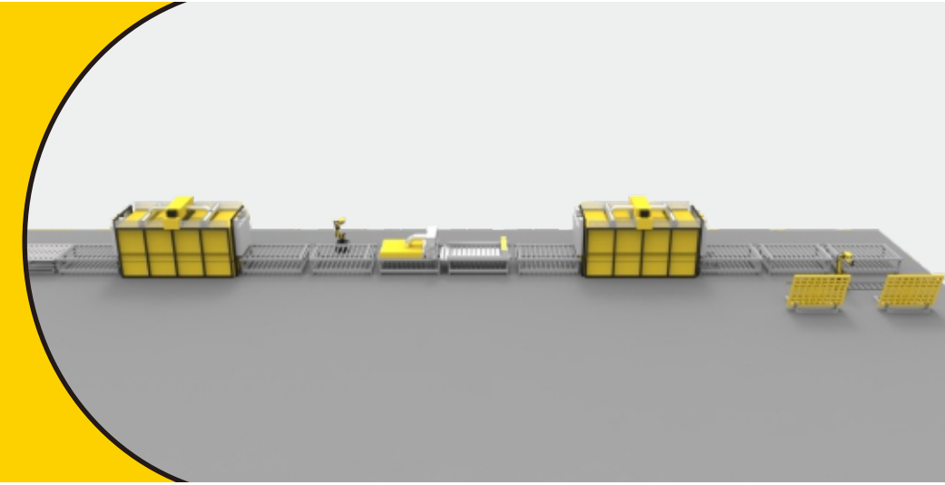
4 Glueing And Drying Of Stone Slabs 大板补胶与烘干设备
