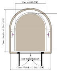
Horseshoe shaped sightseeing elevator (automatic exterior door)
