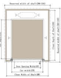
Shaft plan for Manually operated door
