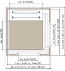
Backpack rack (right angle opening)
