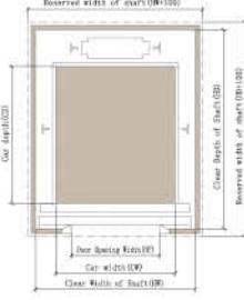
Shaft plan for Center-opening bi-folding door
