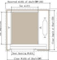
Shaft plan for Side opening door
