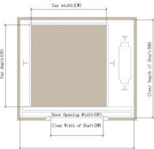
Shaft plan for Center opening door
