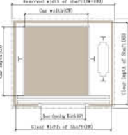
Shaft plan for Center opening door
