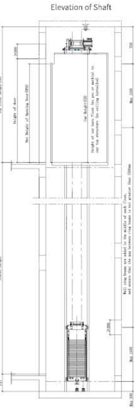
FT (steel belt side-counterweight)
