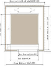
Shaft plan for Side opening door
