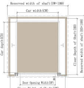
Shaft plan for the Top-mounted drum drive
