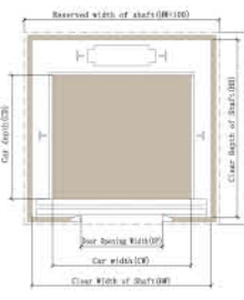
Shaft plan for Center opening door
