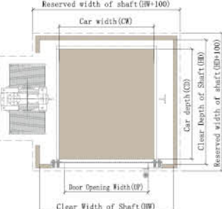
Shaft plan for the Downward drum drive
