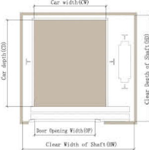
Shaft plan for Side opening door
