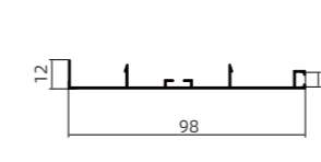
NBW-100 锡脚线 Tin Foot Rail
