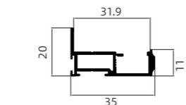
WZB-115 极简移门竖框 Minimalist Sliding Door Vertical Frame
