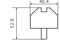
GT18-030 46 双斜层板条 46 Double-Bevel Shelf Strip
