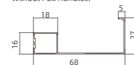
FY-A130 万能外框免拉手 Universal Outer Frame without Pull Handles.
