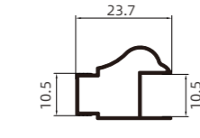
G-024 门框转换条 Door Frame Transition Strip.
