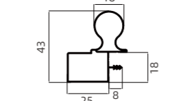
PC-305 小圆弧通体拉手 Small Arc Integrated Pull Handle
