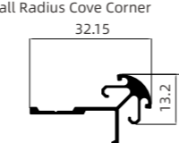
HQB-014 小圆弧阳角 Small Radius Cove Corner
