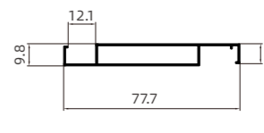
NBW-579 10 厘格栅装饰面板 10mm Grille Decorative Panel
