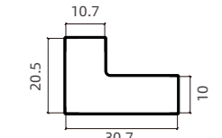
NBW-A005 32 横框 32mm Horizontal Frame.
