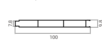
PC-G-112 10 厘扣板 10mm Snap-on Panel.
