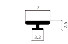
NBW-348 70 装饰条 70mm Decorative Strip.
