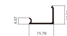
FY-A104 免开铰链孔后盖 Hinge Hole-Free Rear Cover.
