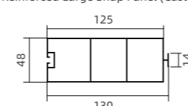
NBW-101 加厚大扣板 (定制) Reinforced Large Snap Panel (Custom)
