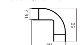
NBW-345 北欧大圆弧框 Nordic Large Arc Frame
