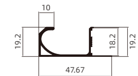
JSLY-013 免铣槽 G 型拉手 Milling-Free G-shaped Pull Handle.
