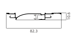
HQB-015 灯槽 Light Trough
