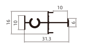
WZB-117 极简移门中隔 Minimalist Sliding Door Center Partition
