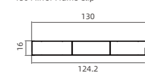
NBW-116 130 镜框扣 130 Mirror Frame Clip
