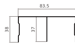
NX-A036 移门上轨 Sliding door top track.
