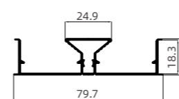
FY-A108 中腰拉手 Waist-high Pull Handle.
