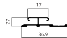
HQB-010 拼接条 Splicing Strip
