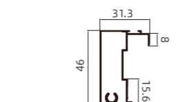
WZB-118 极简移门下方 Minimalist Sliding Door Lower Rail
