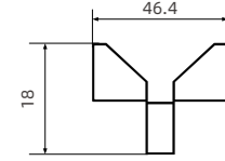
GT18-029 46Y 型层板条 46 Y-Type Shelf Strip
