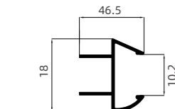
NBW-336 55 平板门框转换条 55mm Flat Door Frame Transition Strip.
