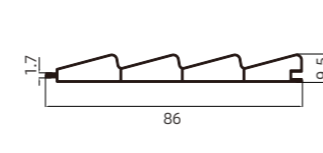
PC-CMJ-A014 四叶百叶板 Four-Blade Louvered Panel.
