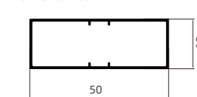
壁厚 Thickness:0.8mm 米重 weight:0.298kg/m
