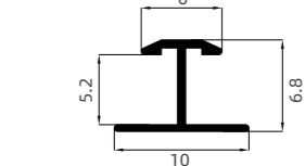
G-064 5 厘工字条 5mm I-Beam Strip.
