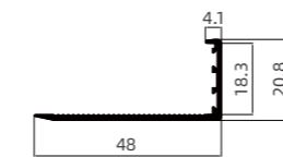
FY-A105 L 型窄边门框 L-shaped Narrow Edge Door Frame.
