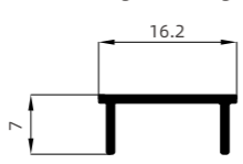
NBW-16-06 16 内封边 16 Internal Edge Banding
