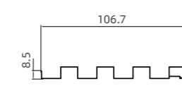
HQB-016 9厘板格栅 9mm Board Grille
