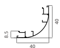
HQB-011 外圆弧阳角 External Radius Cove Corner
