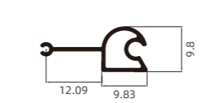
G-116 10 厘圆弧格栅条 10mm Rounded Grille Strip
