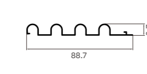
NBW-594 10 厘圆弧格栅板 10mm Rounded Grille Panel
