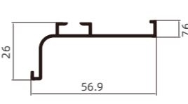
H-1269 下柜拉手 Lower Cabinet Pull Handles
