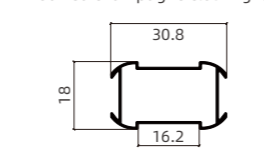
NBW-374 氧化香槟衣通管 Anodized champagne clothing rail tube.
