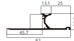
FY-A106 L 型拉手 L-shaped Pull Handle.
