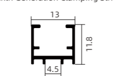
NBW-18-005 第六代卡条 Sixth Generation Clamping Strip
