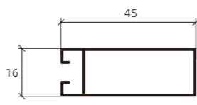
NBW-108 45 背板扣 45 Back Panel Clip
