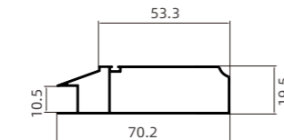
NBW-344 70 装饰门框 70mm Decorative Door Frame.
