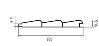
NBW-112 百叶板 Louvered Panel.
