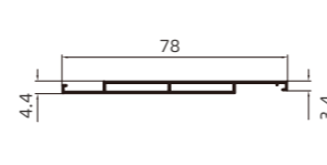
5 厘格栅装饰面板 5mm Grille Decorative Panel
