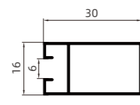
NBW-131 30 背扣板 30mm back strike plate.
