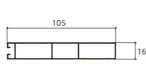
NBW-195 105 背板扣 105 Back Panel Clip
