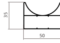
NBW-386 免拉手横拉 Pull-Free Horizontal Sliding Handle
