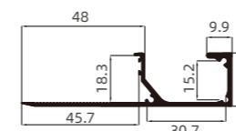
FY-A107 G 型拉手 G-shaped Pull Handle.
