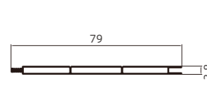
NBW-150 4 厘背板 4mm Back Panel
