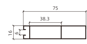
NBW-118 75 背板扣 75 Back Panel Clip
