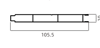
NBW-002 10 厘拼板 10mm Interlocking Panel.
