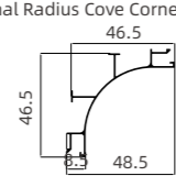
HQB-013 内圆弧阴角 Internal Radius Cove Corner
