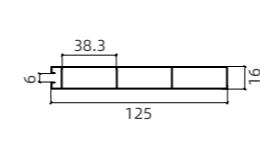
NBW-115 125 背板扣 125 Back Panel Clip
