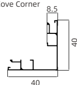
HQB-012 直阳角 Straight Cove Corner
