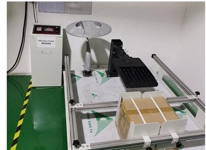
Vibration Test
