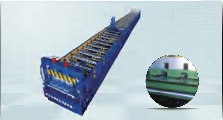
TX50-200-600 闭口式楼承板冷轧成型机 TX50-200-600 closed deck floor board cold rolled shaping machine
