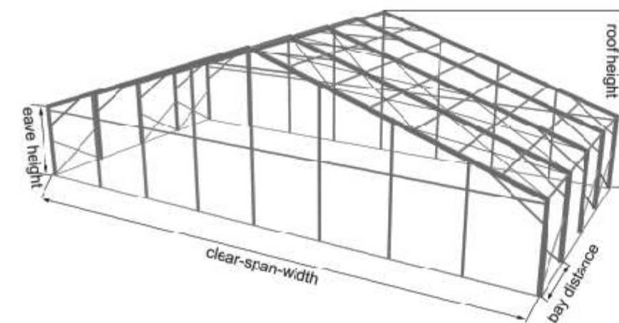
DP series structure specification:
