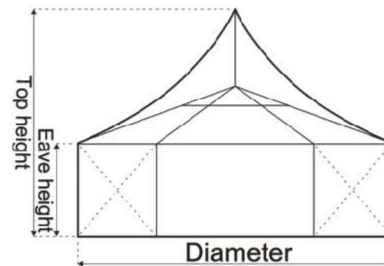
PJ series structure specification:
