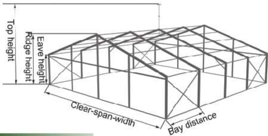
MT series structure specification:
