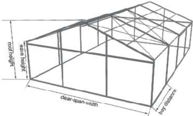
XP series structure specification:
