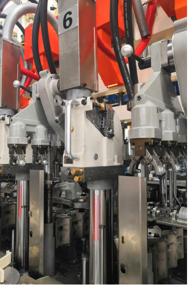
Z270 for Glass Determinant clamp bottle machine
