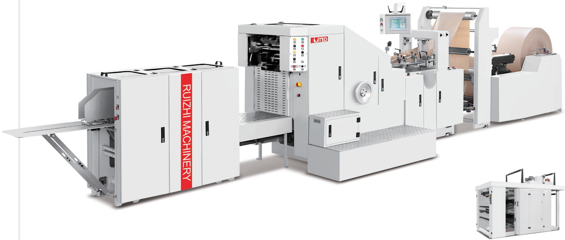
连体印刷机 Siamese Printing Presses
