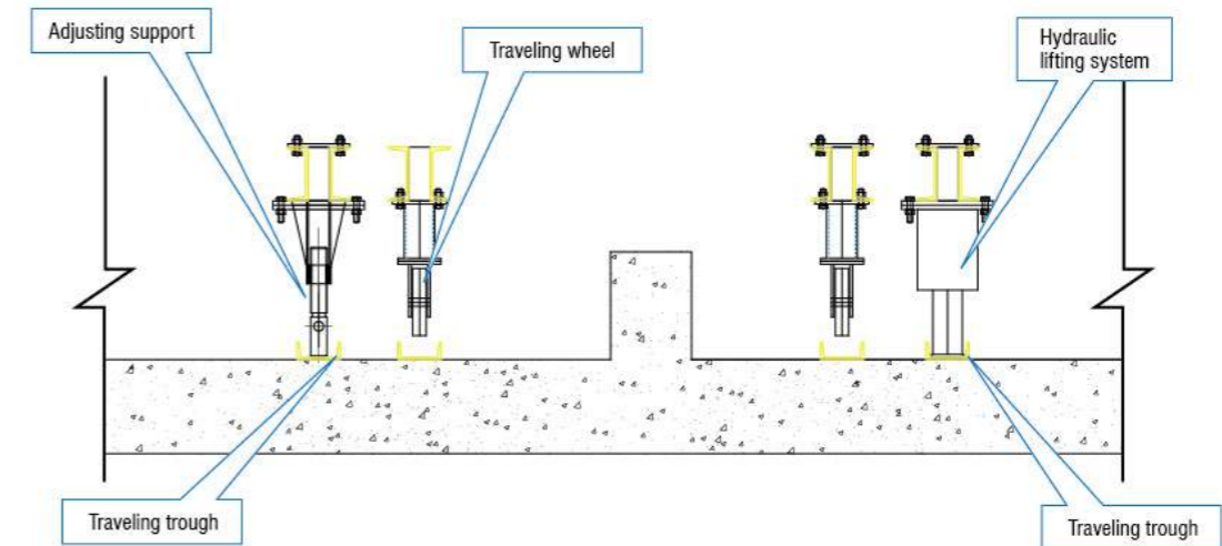
Installation diagram of the bottom stringer
